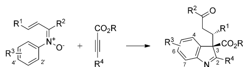
Scheme 2. Reaction of \alpha,\beta -unsaturated N -aryl ketonitrones and activated alkynes.
